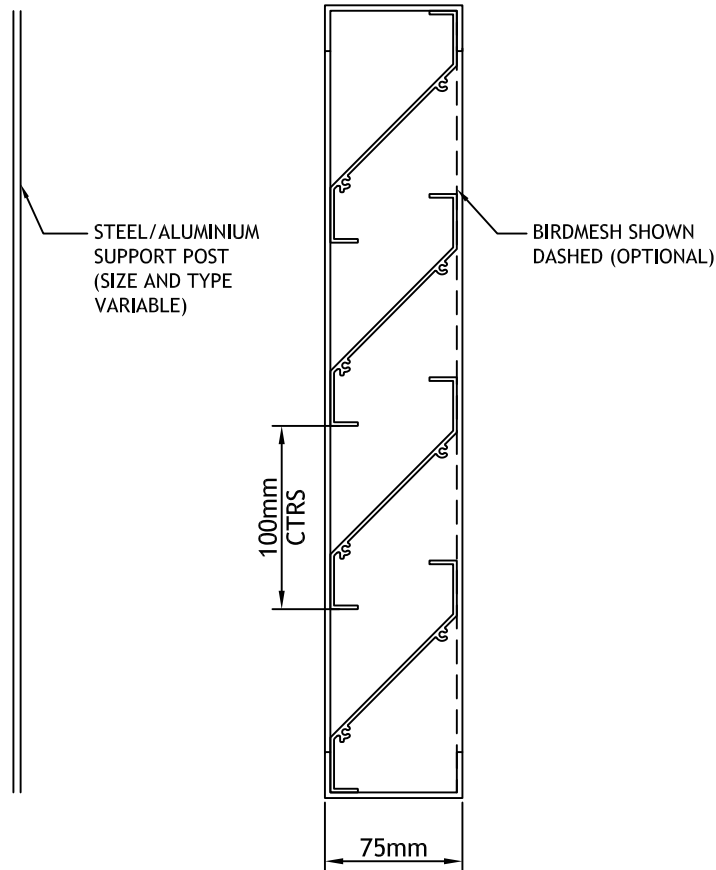
CHANNEL FRAME VERTICAL SECTION
