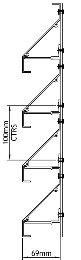
CLIP BRACKET SYSTEM VERTICAL SECTION
