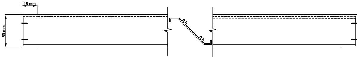
CHANNEL FRAME - HORIZONTAL SECTION
