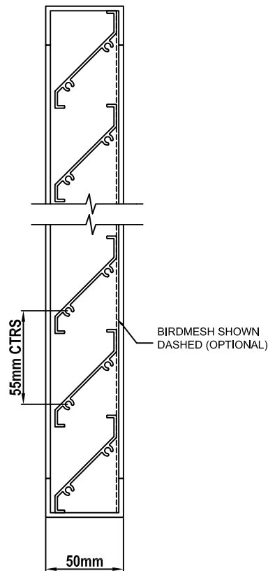
CHANNEL FRAME VERTICAL SECTION
