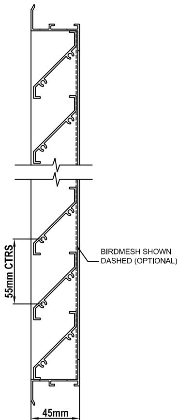
FLANGED FRAME VERTICAL SECTION
