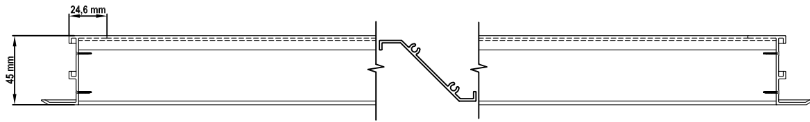
FLANGED FRAME - HORIZONTAL SECTION
