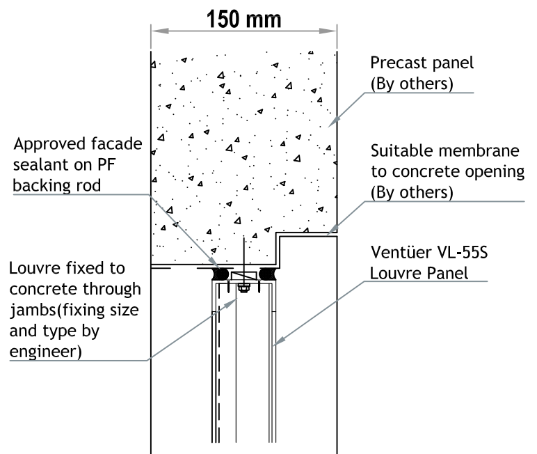
VN-55 (CHANNEL FRAME) JAMB DETAIL 02 SCALE 1 : 4
