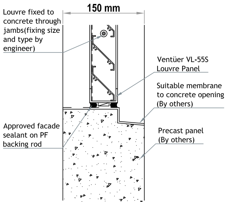
VL-55S (CHANNEL FRAME) SILL DETAIL 03 SCALE 1 : 4
