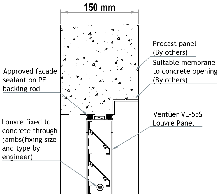
VL-55S (CHANNEL FRAME) HEAD DETAIL 01 SCALE 1 : 4
