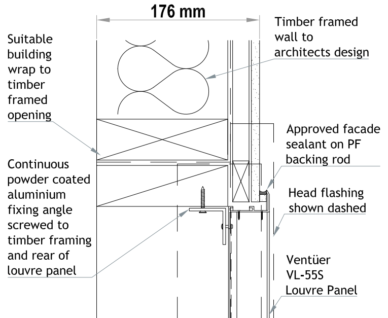
VL-55S (FLANGED FRAME) JAMB DETAIL 02 SCALE 1 : 4
