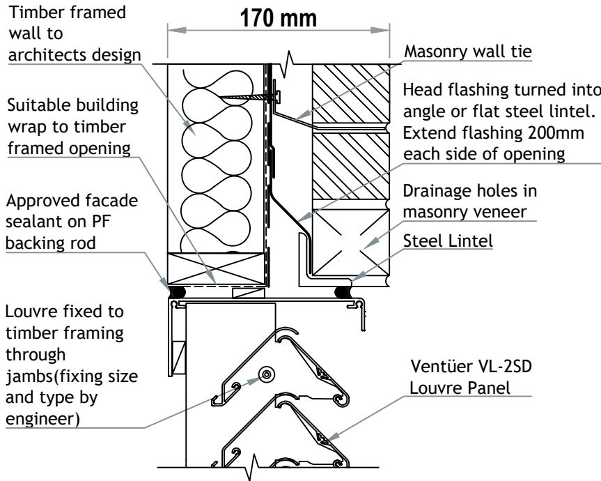
VL-2SD (FLANGED FRAME) HEAD DETAIL 01 SCALE 1 : 4
