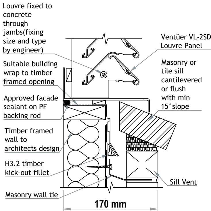
VL-2SD (FLANGED FRAME) SILL DETAIL 03 SCALE 1 : 4
