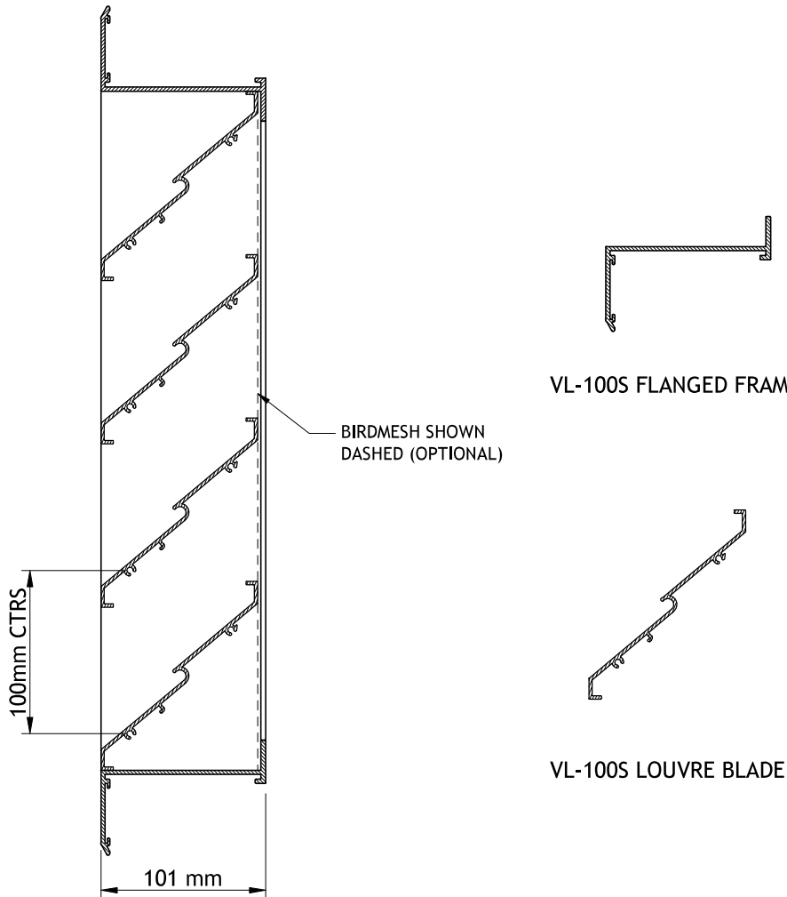
FLANGED FRAME VERTICAL SECTION
