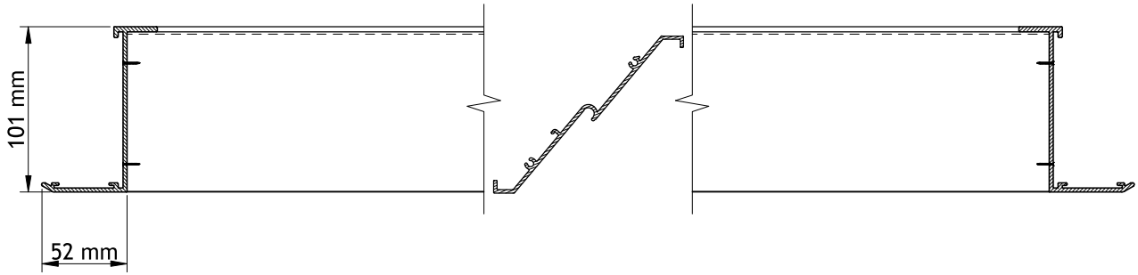
FLANGED FRAME - HORIZONTAL SECTION
