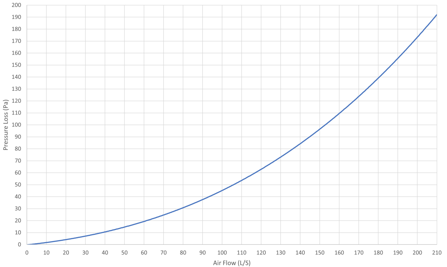
Airflow Performance - 150mm Stainless Steel Cowl with Insect Mesh
