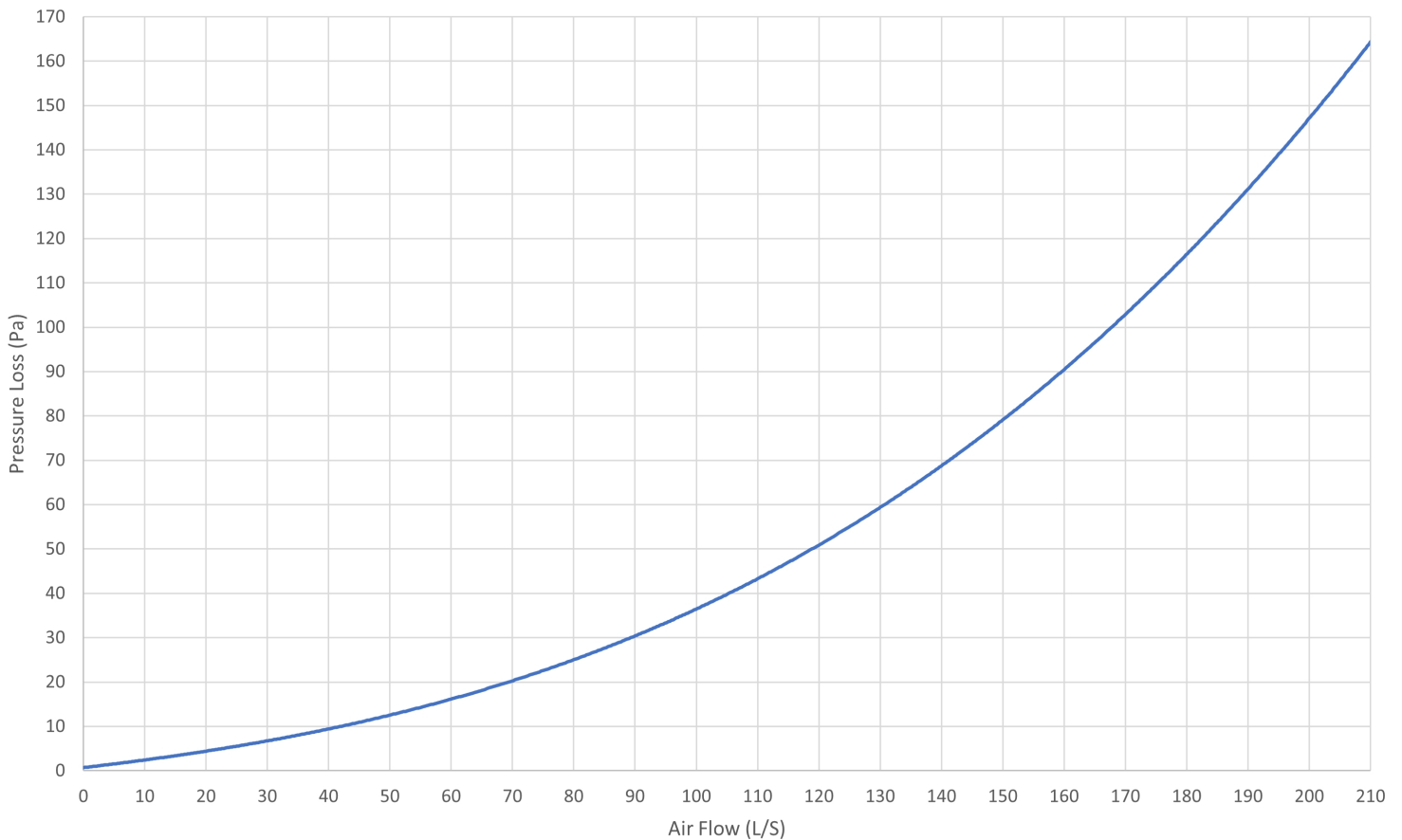
Airflow Performance - 150mm Stainless Steel Cowl with Backdraft Flap
