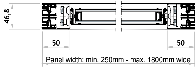
HORIZONTAL SECTION
