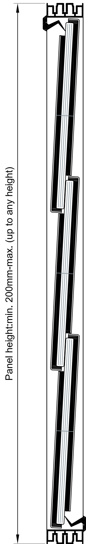
VERTICAL SECTION
