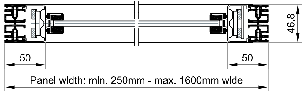
HORIZONTAL SECTION
