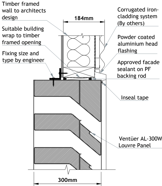
AL-300W (CHANNEL FRAME) HEAD DETAIL 01 SCALE 1 : 8
