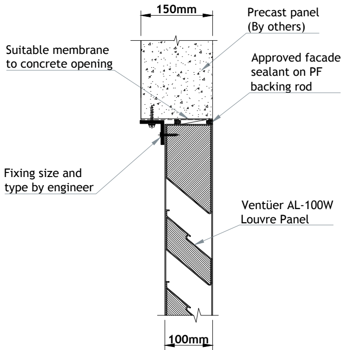
AL-100W (CHANNEL FRAME) HEAD DETAIL 01 SCALE 1 : 8
