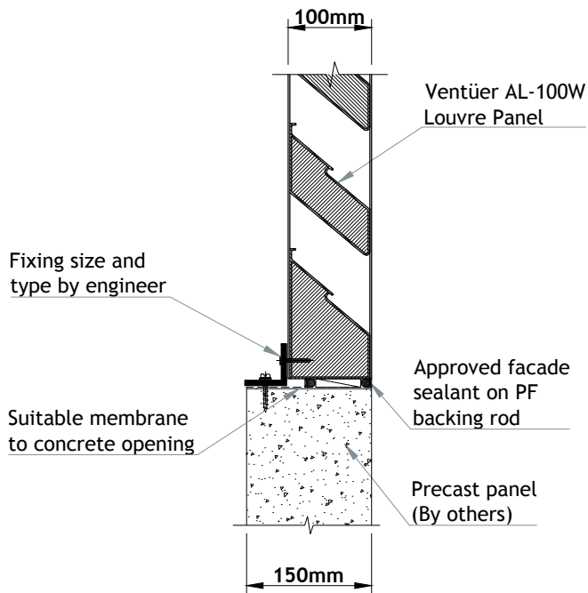
AL-100W (CHANNEL FRAME) SILL DETAIL 03 SCALE 1 : 8
